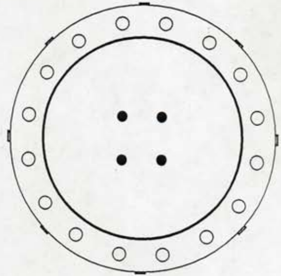
COMPLETION PLUG INSTALLED UNDER PRESSURE (TOP VIEW)
